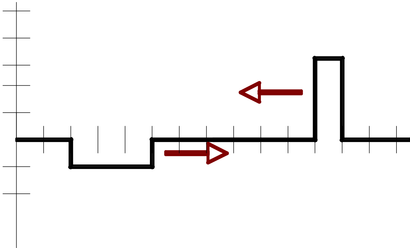
Wave addition simple pulse
